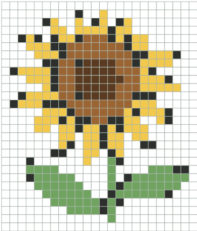
MOSAIC ANSWER
